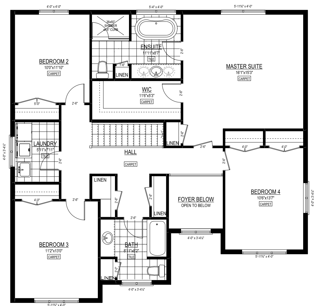
SECOND FLOOR 1394 SQ.FT
