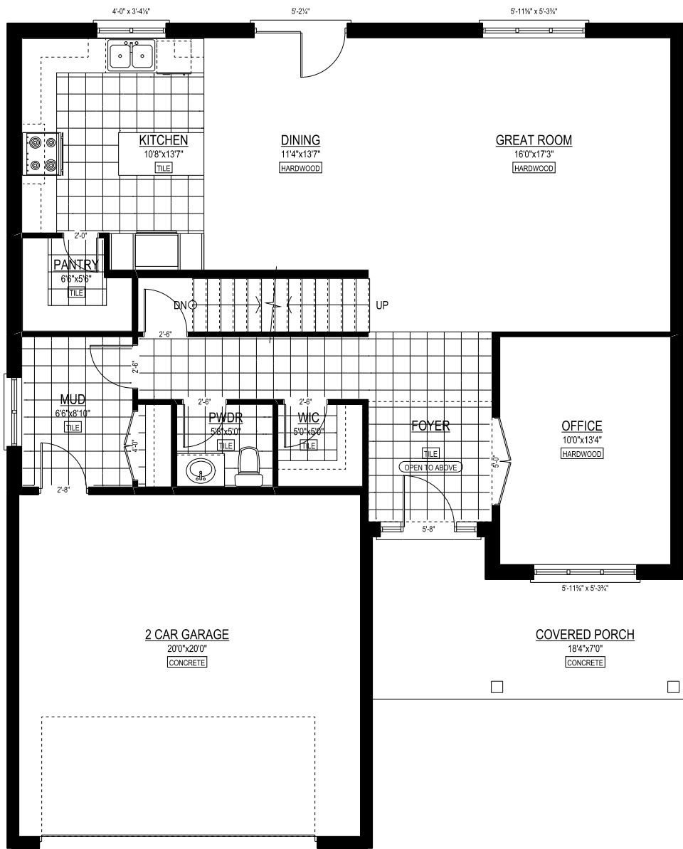
MAIN FLOOR 1174 SQ.FT
